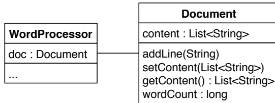
Figure 4.4: Example application, used throughout this chapter
