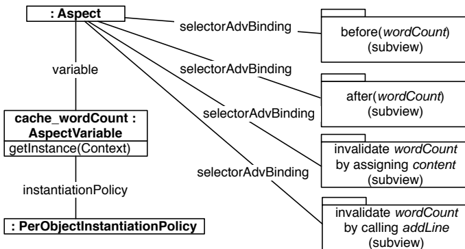
Figure 4.12: Mapping a caching aspect to JAMI concepts
