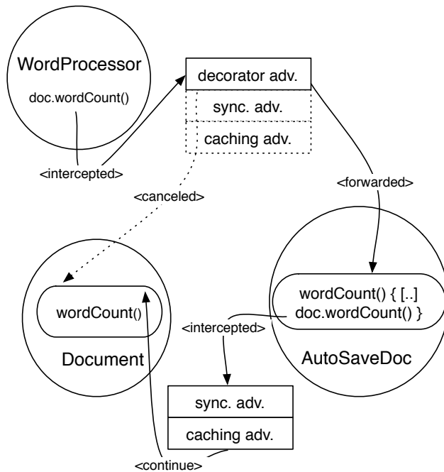
Figure 4.17: Control flow combining aspects from 3 DSALS
