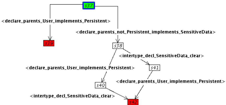
Figure 3.18: Transformation state space: applying introductions in different orders
