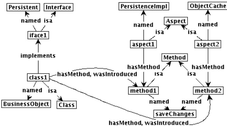
Figure 3.8: Final program model after applying introductions
